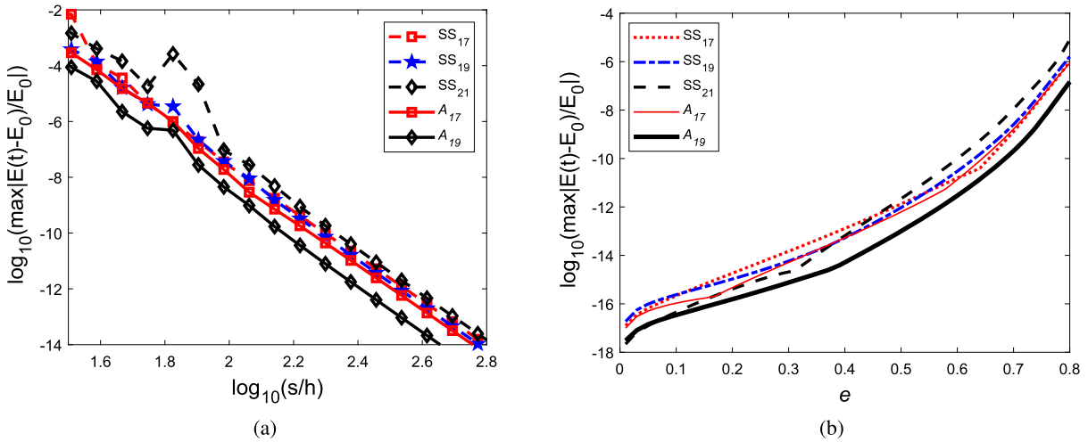
Fig. 3. (a) Efficiency diagram for the Kepler problem with e = 0.5 for composition SS_m and the new RKN splitting methods A_{17} and A_{19} . Final time t_f = 1000 . (b) Maximum error in energy for different values of the eccentricity with t_f = 1000 and s/h = 340 .
